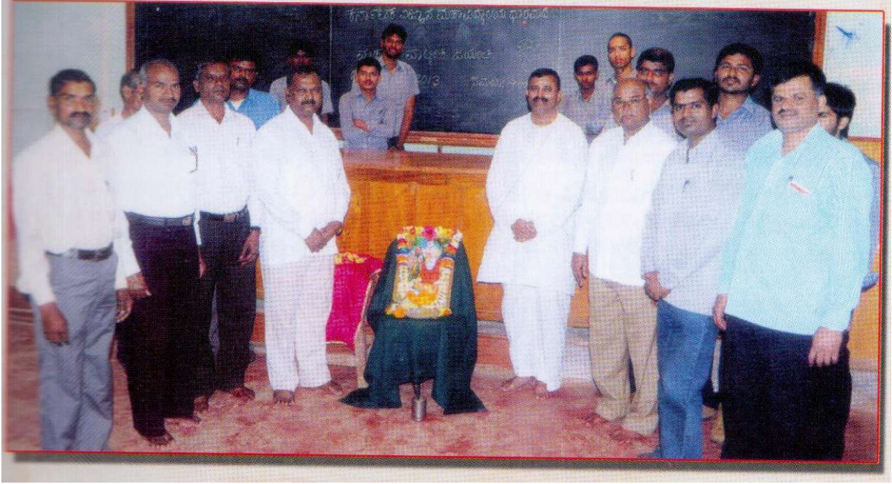
Walmiki jayanti
